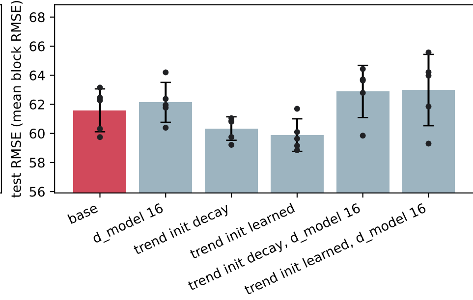
trend blend: test
